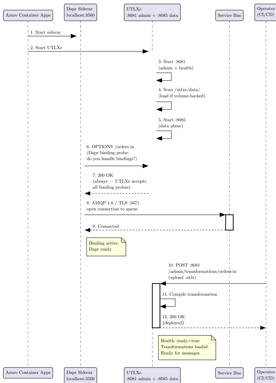
Figure 1: Startup sequence: Dapr probe, Admin API upload, then ready for messages
